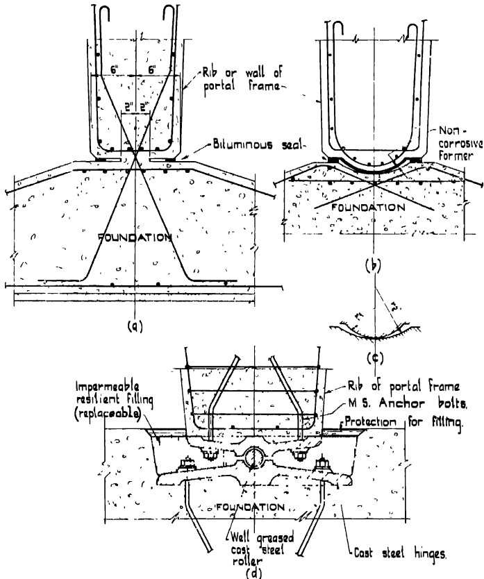
Fig. 335.—Hinges for Portal Frames.
